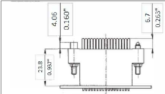
Header Dimensions Straight Standard Profile Header
