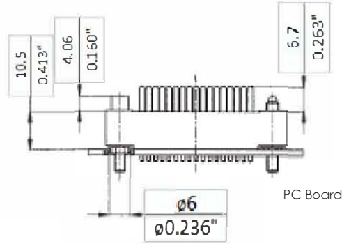
Header Dimensions Straight Low Profile Header
